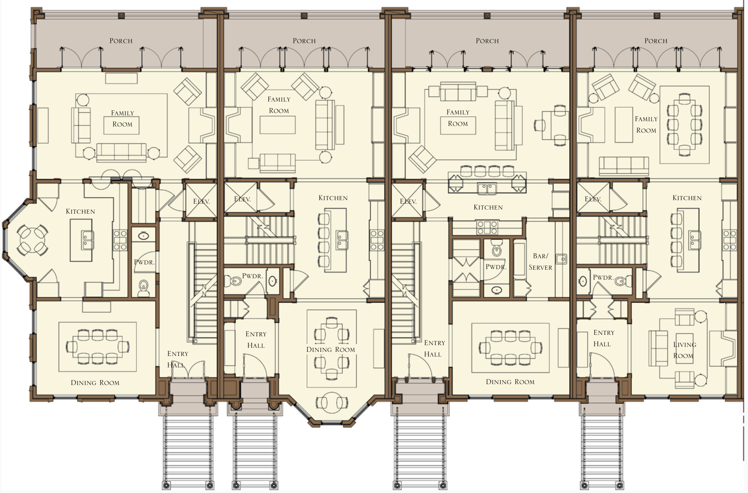
MAIN LEVEL FLOOR PLAN
