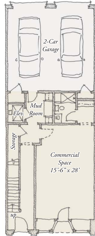
Ground Floor Option B 900 S.F.
