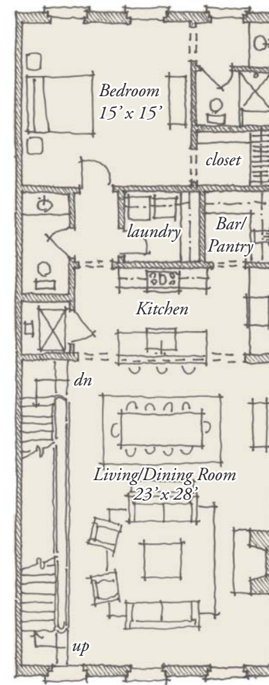
Main Level 1,440 S.F.
