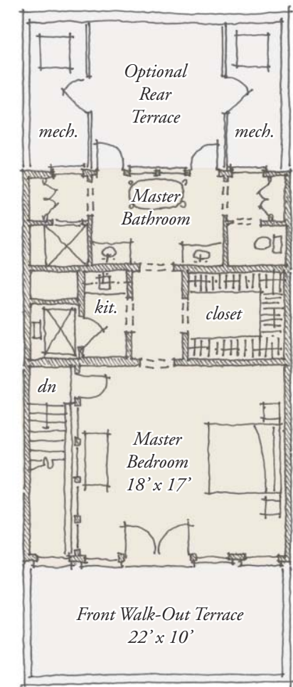
Upper Level 840 S.F.
